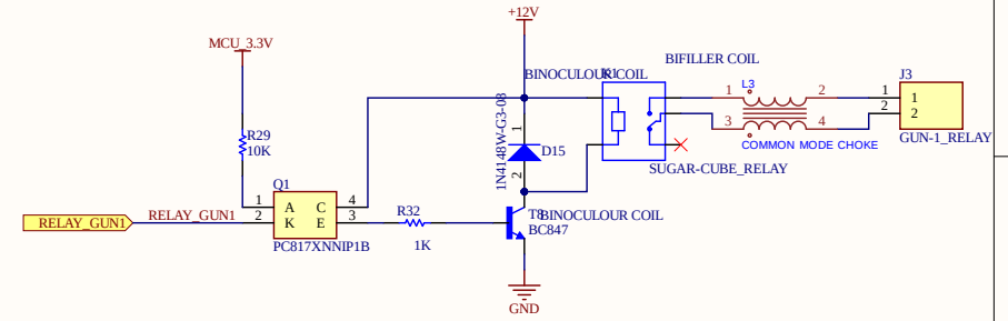
GUN-1_RELAY
