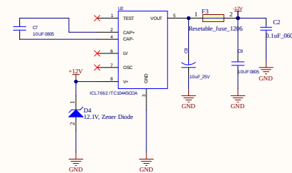
Negative 12V generation Circuit
